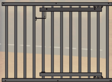
EQBW425548400SP 48" x 34 5/8" WALL GRILL with FEED DOOR 1" TUBES @ 4" o.c. BLACK WELDED
