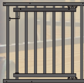
EQBW425536400SP 36" x 34 5/8" WALL GRILL with FEED DOOR 1" TUBES @ 4" o.c. BLACK WELDED
