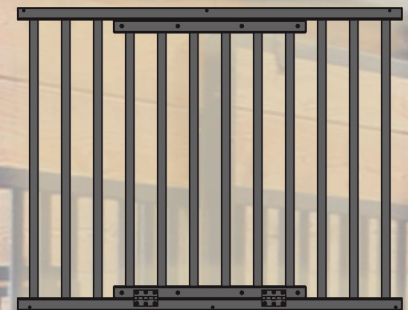
EQBW430148400SP 48" x 36" WINDOW DROP GRILL 1" TUBES @ 4" O.C. BLACK WELDED
