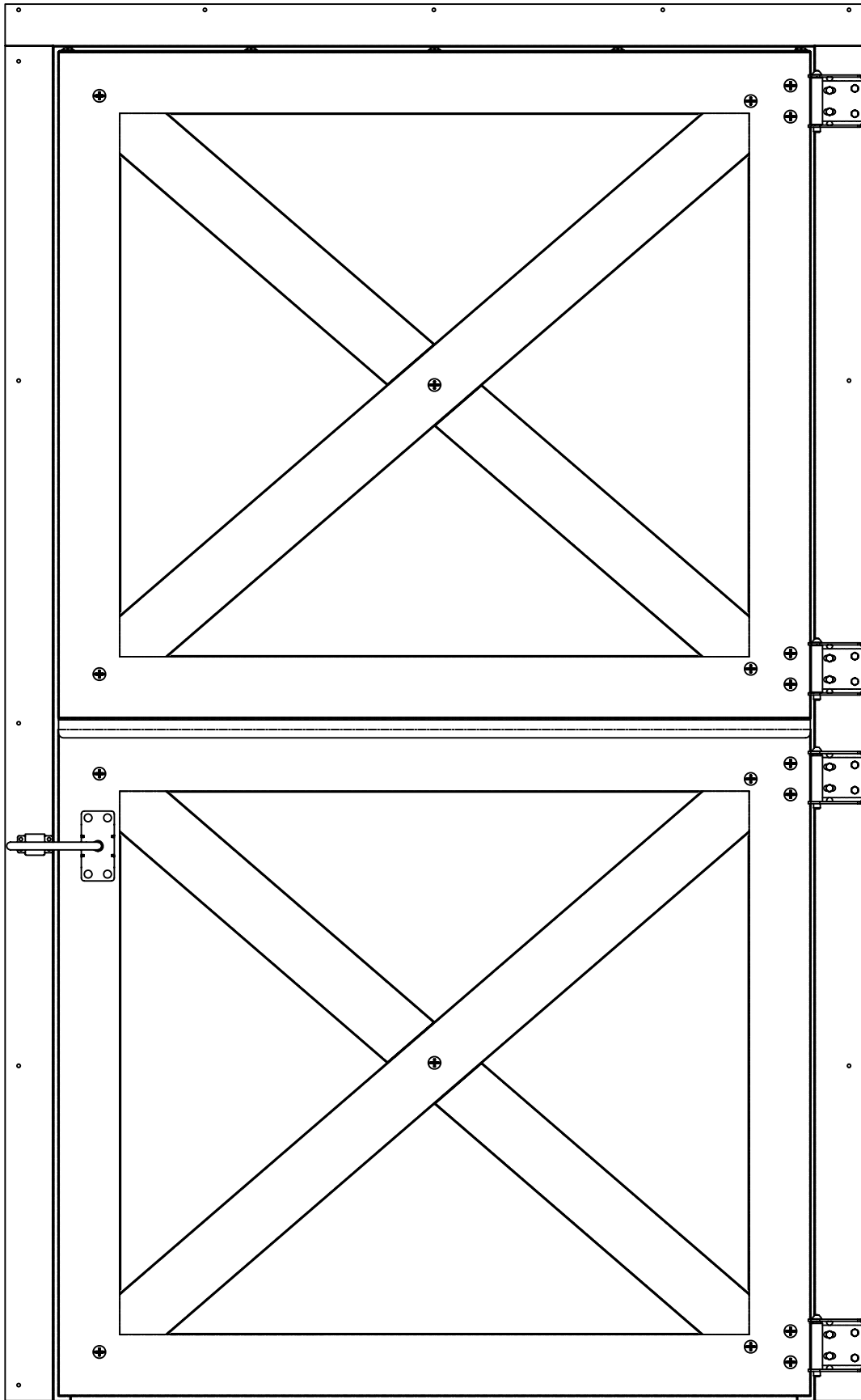
MODEL 4700 - ASSEMBLED PANELS / KD FRAME - 4/0 X 7/0 PLYCO CORPORATION - ELKHART LAKE, WI 53020 - 800-558-5895
