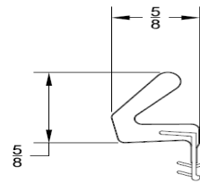
Compression Jamb Seal
