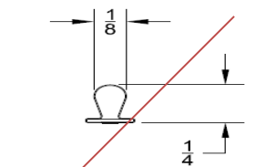
99 BULB SEAL WS-014
