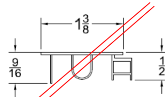
OLD 92 SWEEP
