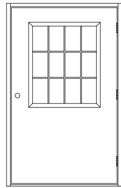
12-LK-2 30x36 Insulated 12 Lite (Series 20 4/0 Doors)
