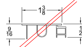
OLD 92 SWEEP WS-001
