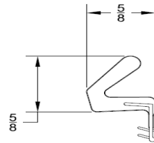
Compression Jamb Seal WS-011
