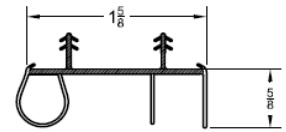
EVERLAST SWEEP WS-006E Current as of Nov. 2014 Bottom of Door, used with threshold (fins are removed and double sided tape is added)
