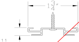
ADA Seal Extension # 1572
