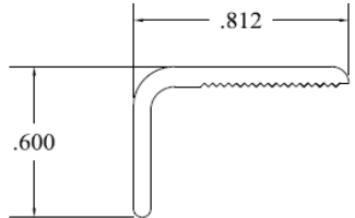
88 Seal Holder WS-013/LO Strike & Hinge Jamb Current (April 2016 - current , used on all doors.)
