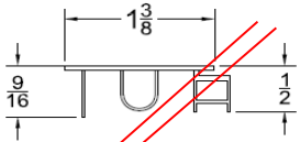
OLD 92 SWEEP WS-001
