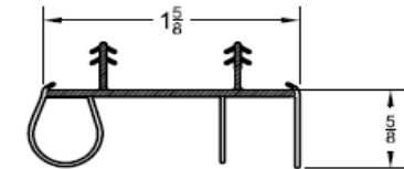
EVERLAST SWEEP WS-006E (All 32 TB May 2013 - current) Bottom of door only
