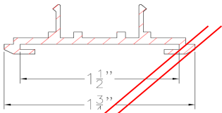
Seal Holder #1276 Obsolete May 2003
