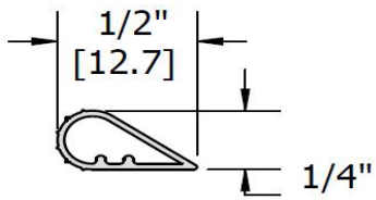
WS-019 Smoke Seal Series 22
