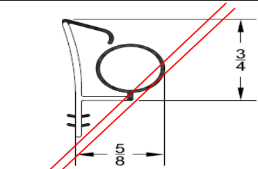
98 JAMB SEAL WS-002 Obsolete 8/2010 No longer available
