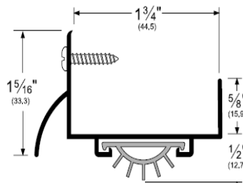
WS-023 Outswing Replacement for outswing doors manufactured before Feb. 2021
