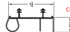
EVERLAST SWEEP - PVC WS-025 Top & Bottom of Doors
