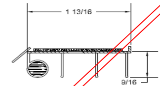
98FG SWEEP Obsolete WS-005 INSWING through 2012 (Feb. 2007 - 2013) No longer available
