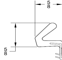
Compression Jamb Seal WS-011
