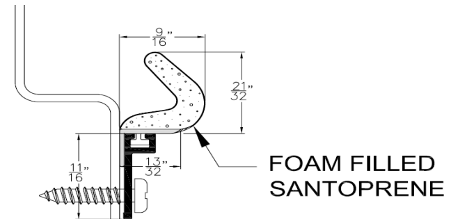
WS-024 Jamb and Header Seal Standard Jamb Seal for Series 23 & 24 & 24T
