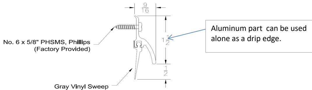
WS-770 SWEEP Standard Sweep - Series 22 & 23
