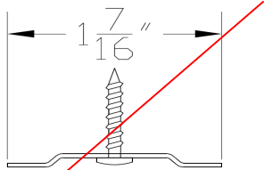
Obsolete Series 20 "Taylor" Seal-holder Most recent (2012) - needed for all WS-020 applications. Bottom of "old" Series 24 doors. ( - 2013)
