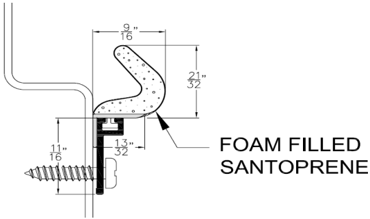
WS-024 Jamb and Header Seal Standard Jamb Seal for Series 23 & 24 & 24T
