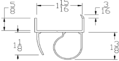
WS-004 Used without threshold
