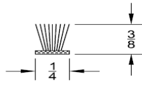
99 FUZZY SEAL WS-012 Wool Pile T-Seal Used on all 99's & 99E's
