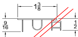
OLD 92 SWEEP WS-001
