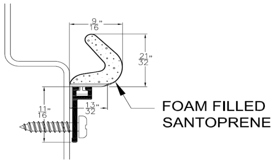
WS-024 Jamb and Header Seal Standard Jamb Seal for Series 23 & 24 & 24T
