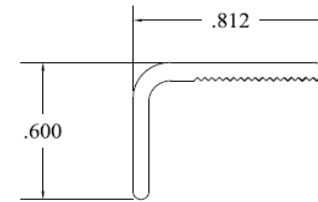
88 Seal Holder WS-013/LO Strike & Hinge Jamb Current (April 2016 - current , used on all doors.)
