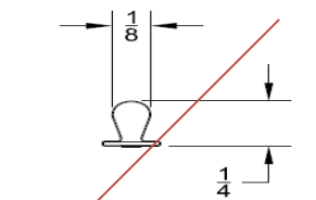
99 BULB SEAL WS-014
