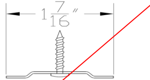
Obsolete Series 32 "Taylor" Seal-holder Most recent (2012) - needed for all WS-020 applications. Bottom of "old" Series 32 OUTSWING doors. Some available for repair
