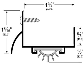
WS-023 Outswing Replacement for outswing doors manufactured before Feb. 2021
