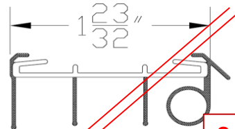
Obsolete WS-020 (2006 - 2013) - works for all "old" Series 32 OUTSWING doors, bottom of door only.
