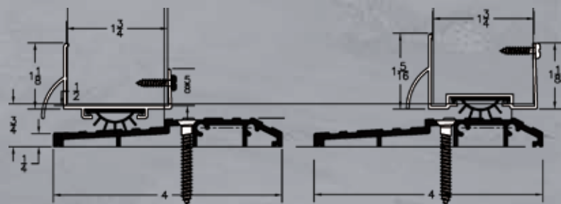
Superior Door Seal System for inswing and outswing doors (Fire rated doors have saddle type threshold)
